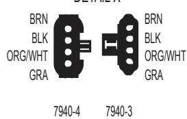
DETAIL X
