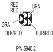
DETAIL T
